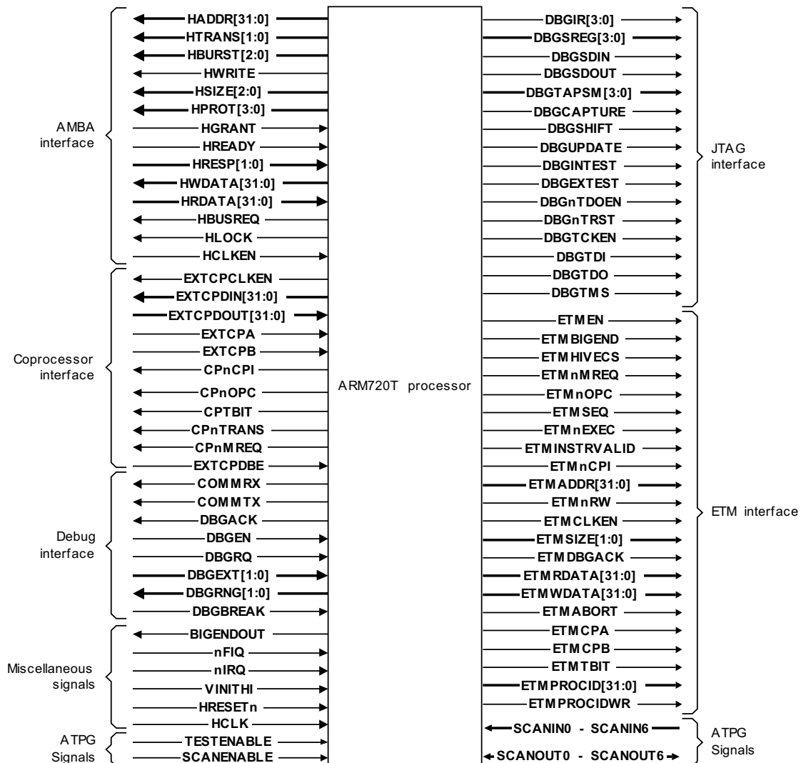
Figure 1-2 ARM720T processor functional signals
